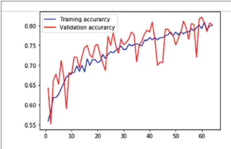
Figure : Training and validation accuracy of our model
