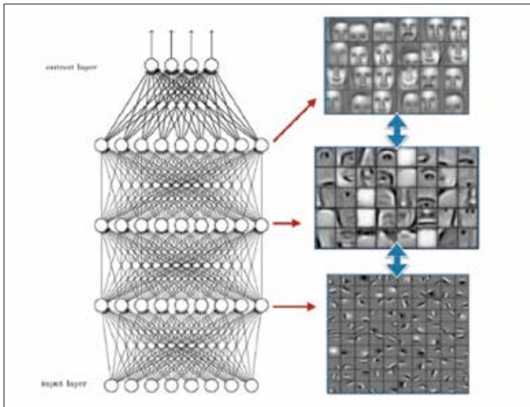
Figure : Neural network learning at increasing levels of complexity
