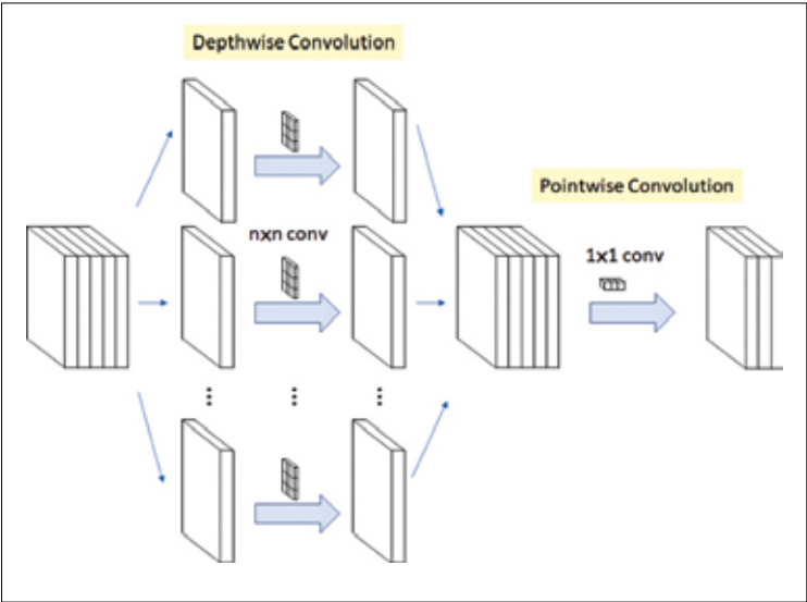
Figure : Depth wise and pint wise convolution
