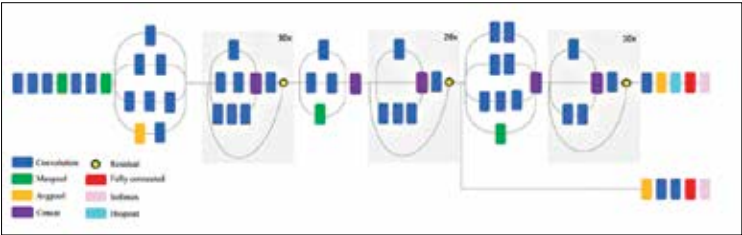
Figure : Inception Resnet V2 model
