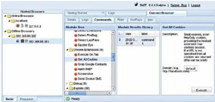
Using commands to get cookies in browsers
