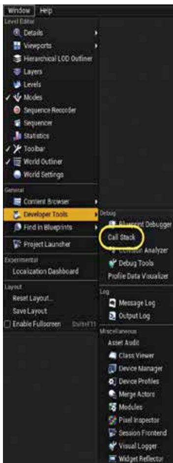
Call Stack
