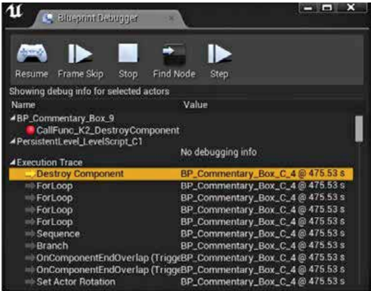
Execution Trace
