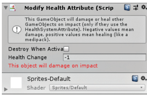
The Modify Health component
