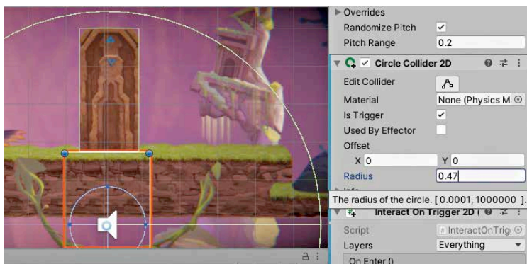
Adding a circle collider to a rectangular door, to trigger the open animation when Ellen walks within the limits of the circle.
