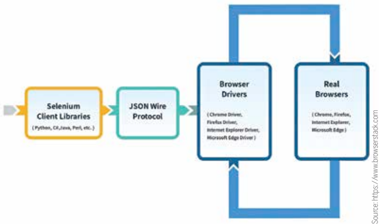
Selenium: Web Architecture
