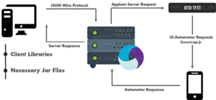
Appium for iOS
