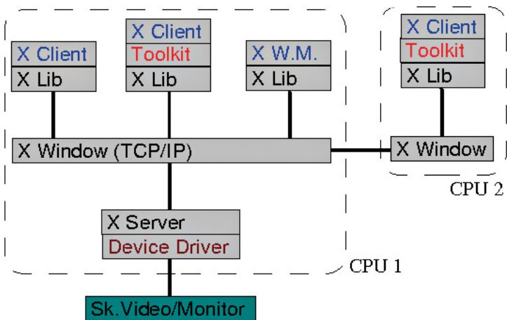
Architecture of X-Window
