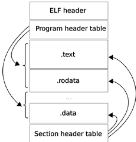
Linux ELF binary header file structure.
