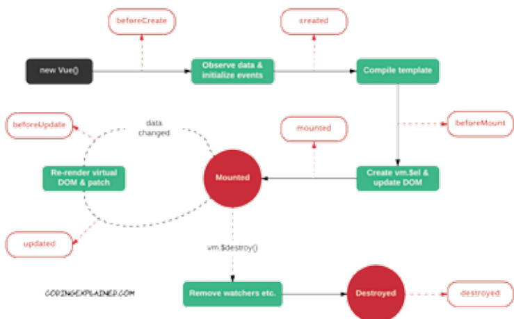
Explanation of Vue instance Lifecycle Hooks
