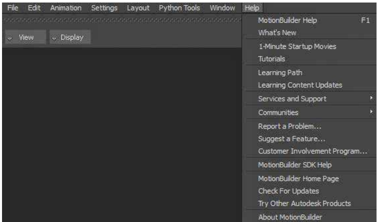
Help Menu
