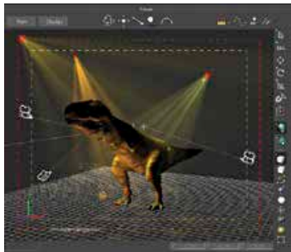
Viewer Window
