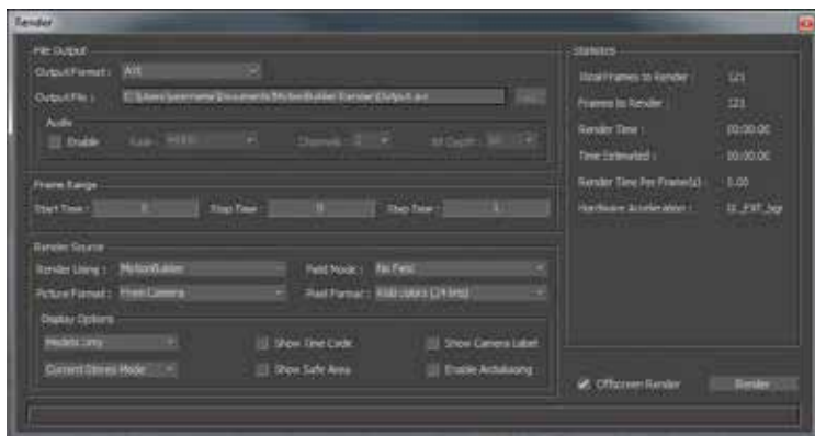
MotionBuilder Render Window
