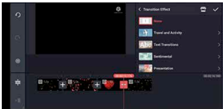
Transition effects
