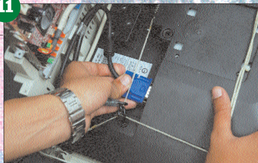
11 Connect everything up—most importantly, remember to connect all LCD connections before you close the CRT case
