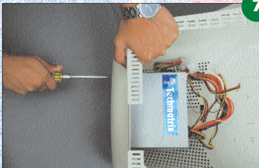
7 Making sure the power supply is firmly held in place. If it falls on the motherboard, that's the end of that!
