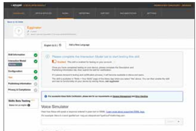
Testing your Alexa skill
