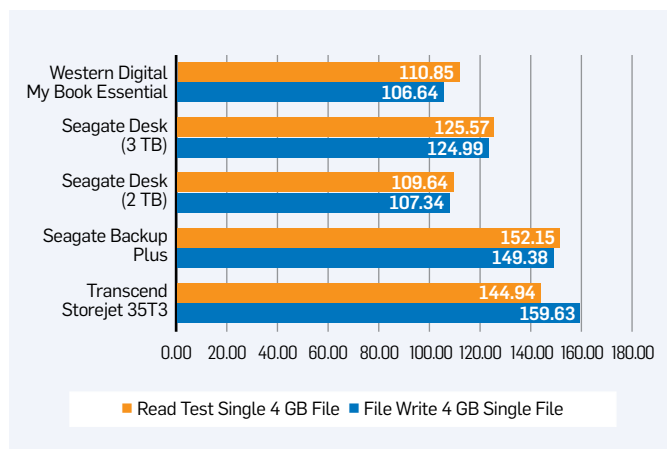
Powered Drives Sequential File Transfer
