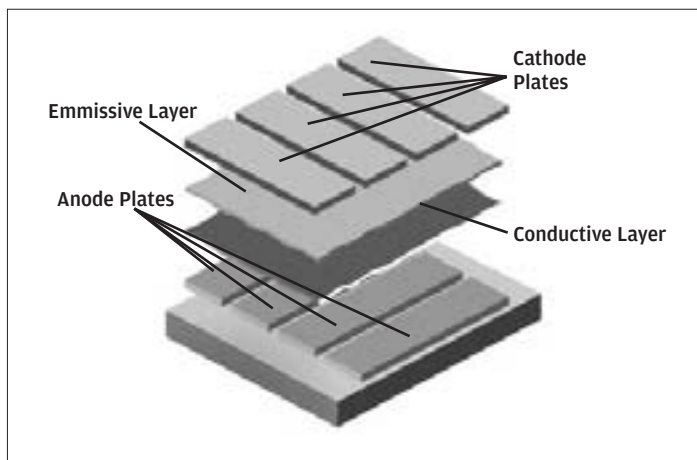
Construction of an OLED
