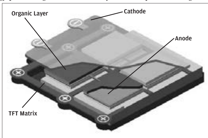
Structure of an Active Matrix OLED
