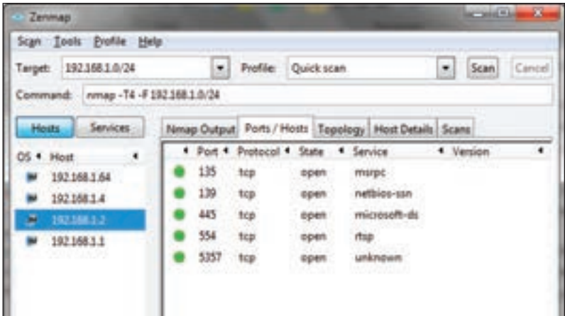
Zenmap showing a list of ports on the selected host (192.168.1.2)
