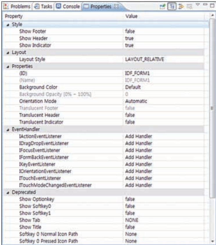
Resource Explorer Properties tab
