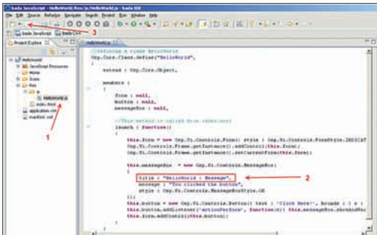
HelloWorld project
