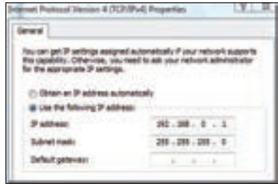
Internet Protocol Version 4(TCP/IPv4) Properties
