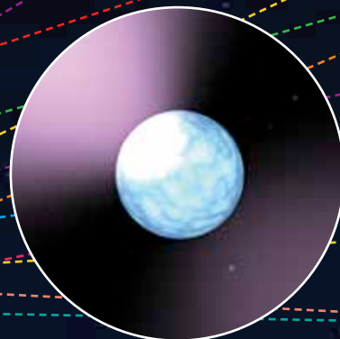
EXPLODING NEUTRON STARS
