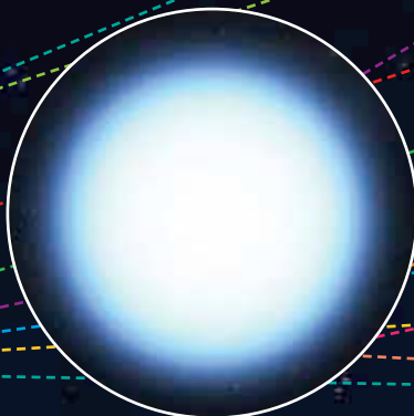
EXPLODING WHITE DWARFS
