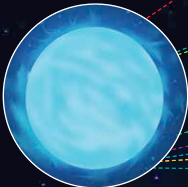
EXPLODING MASSIVE STARS
