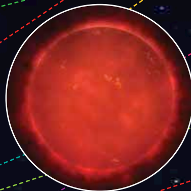
LOW MASS STARS
