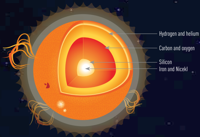
CROSS SECTION OF A SUN LIKE STAR
