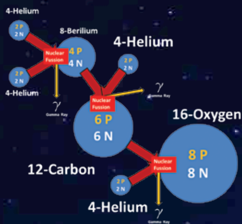
OXYGEN NUCLEOSYNTHESIS
