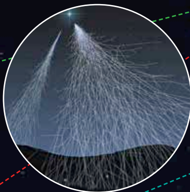
COSMIC RAY SPALLATION
