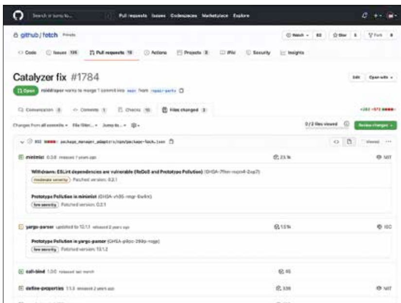
Dependency Review
