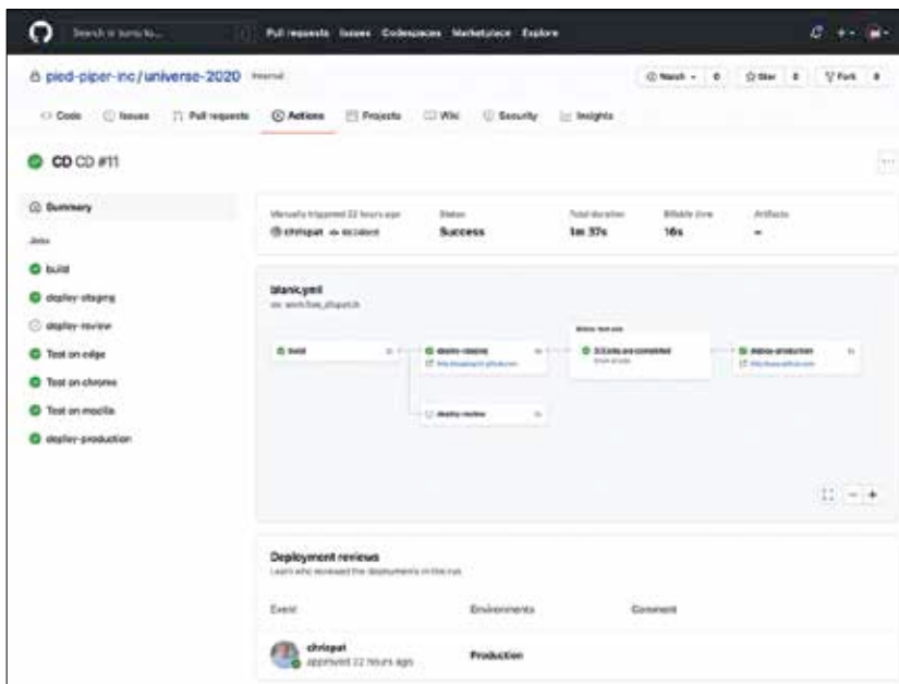
Workflow visualiser
