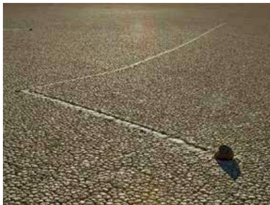
The moving rocks and the trail they left behind
