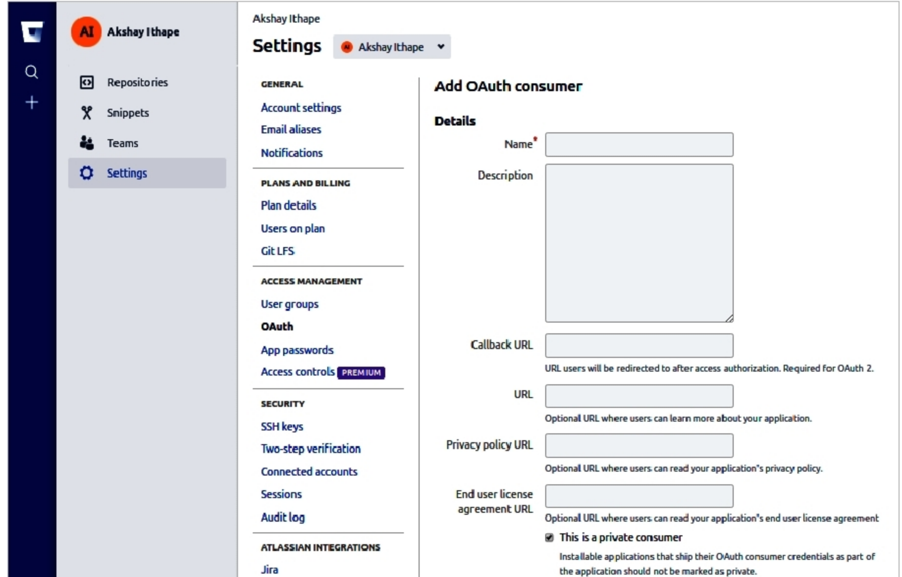
Figure 4: Configuring OAuth in Bitbucket
