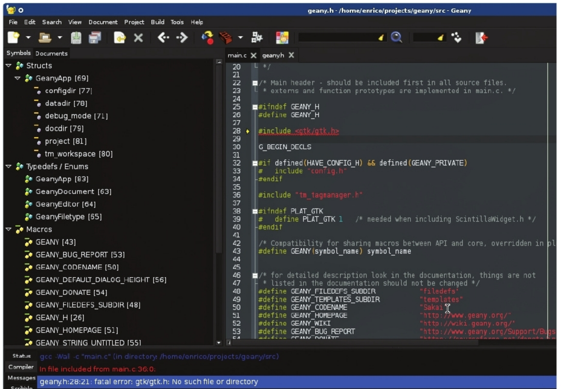
Figure 2: Geany IDE
