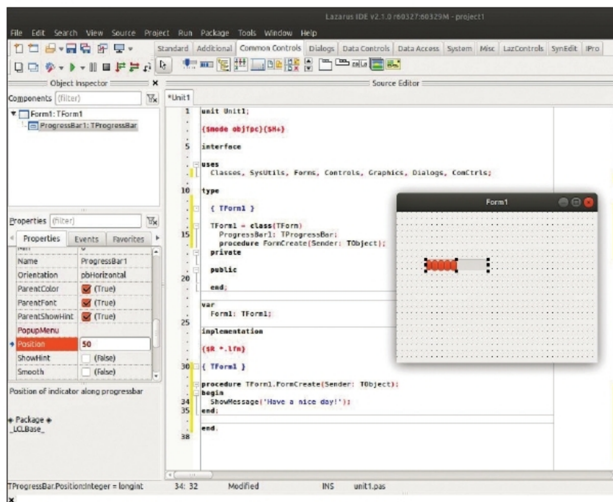
Figure 3: Lazarus IDE
