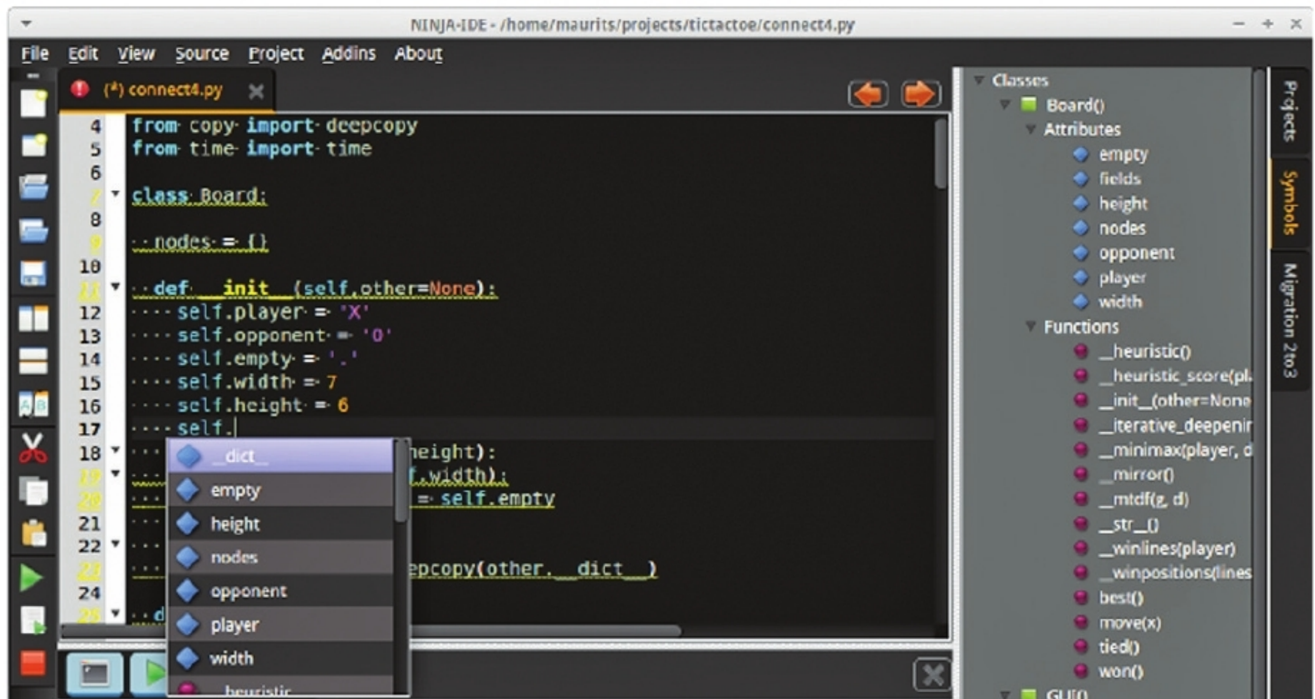
Figure 6: Ninja IDE
