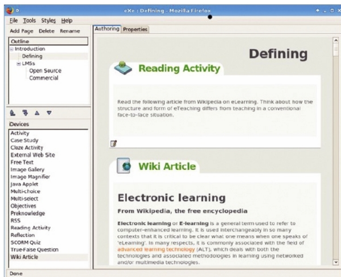
Figure 5: exeLearning
