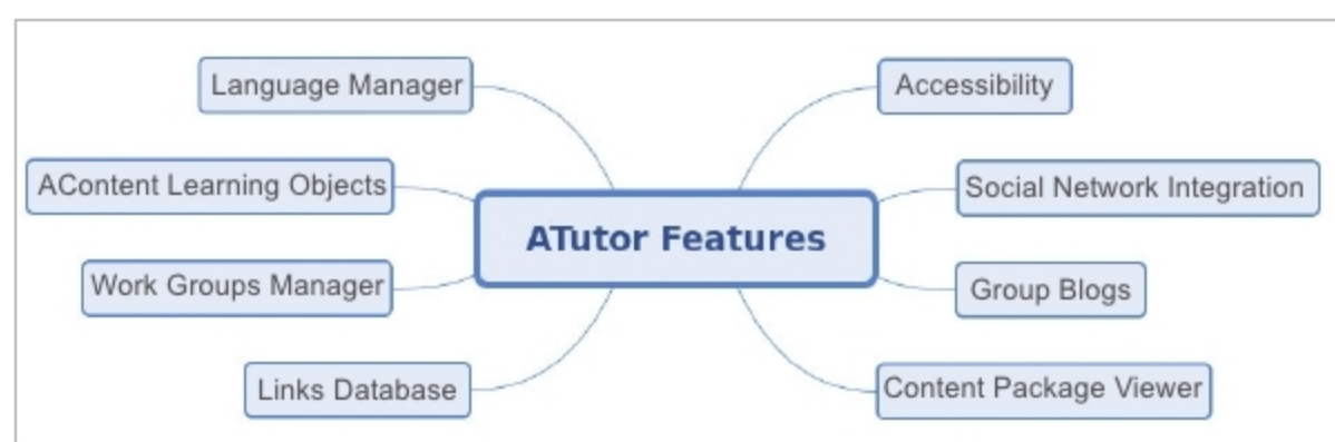
Figure 4: ATutor's features
