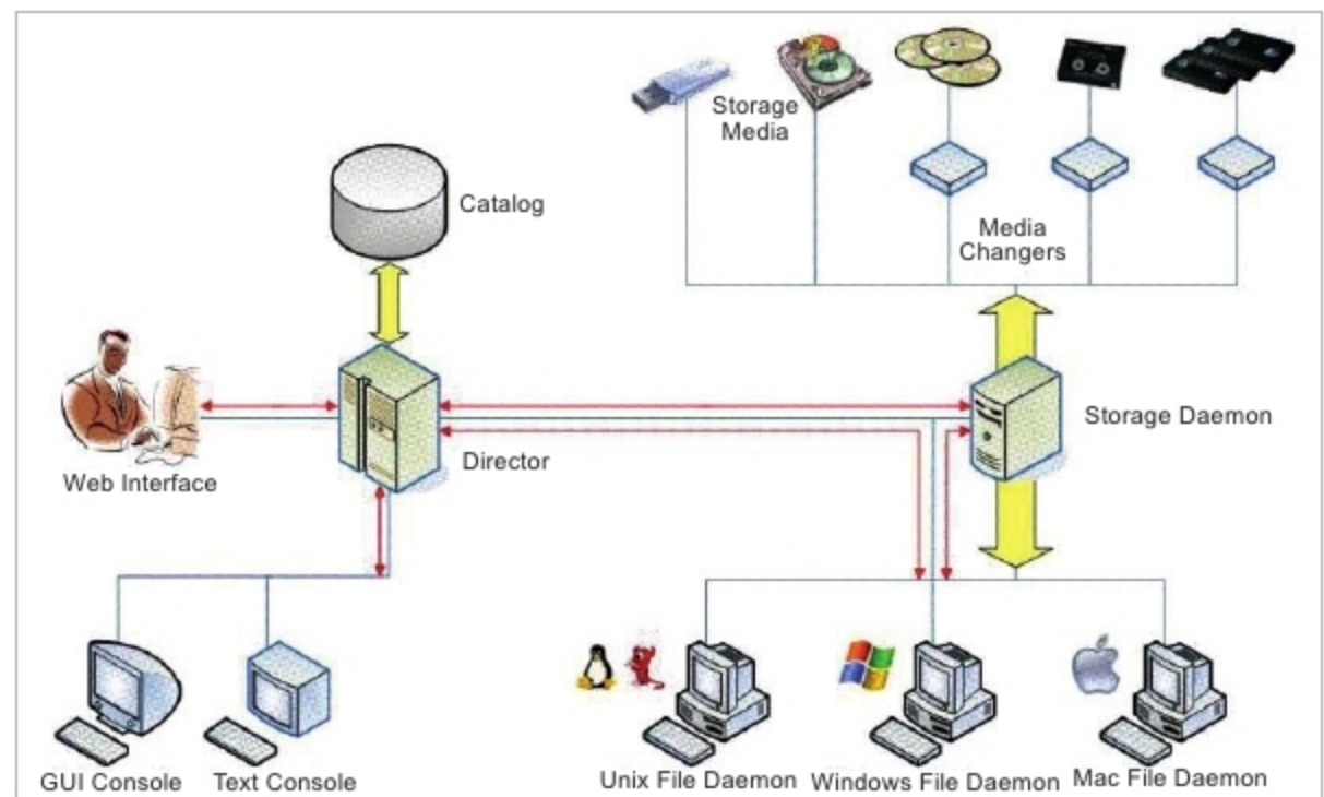
Figure 1: Bacula's components
