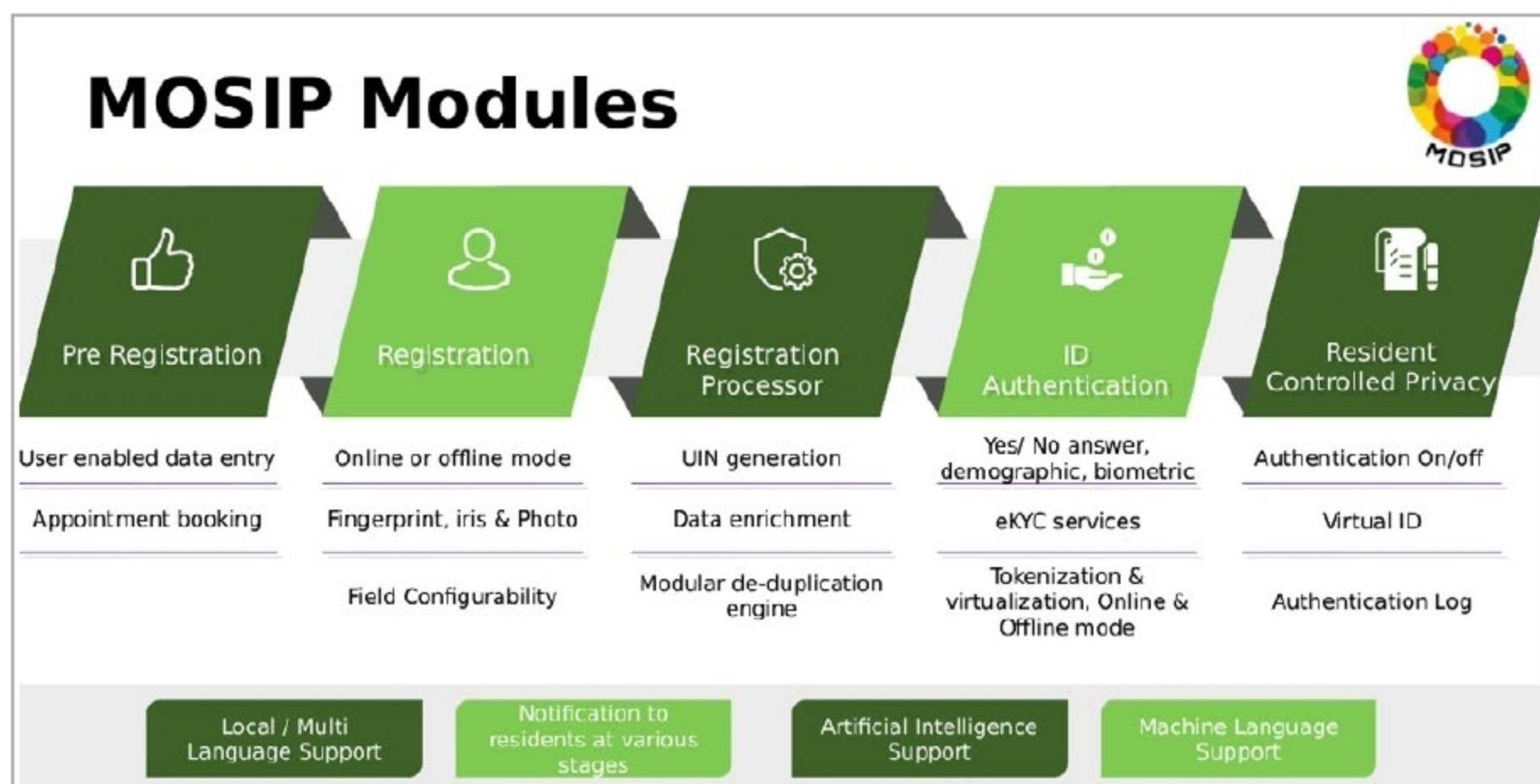
Figure 2: MOSIP modules
