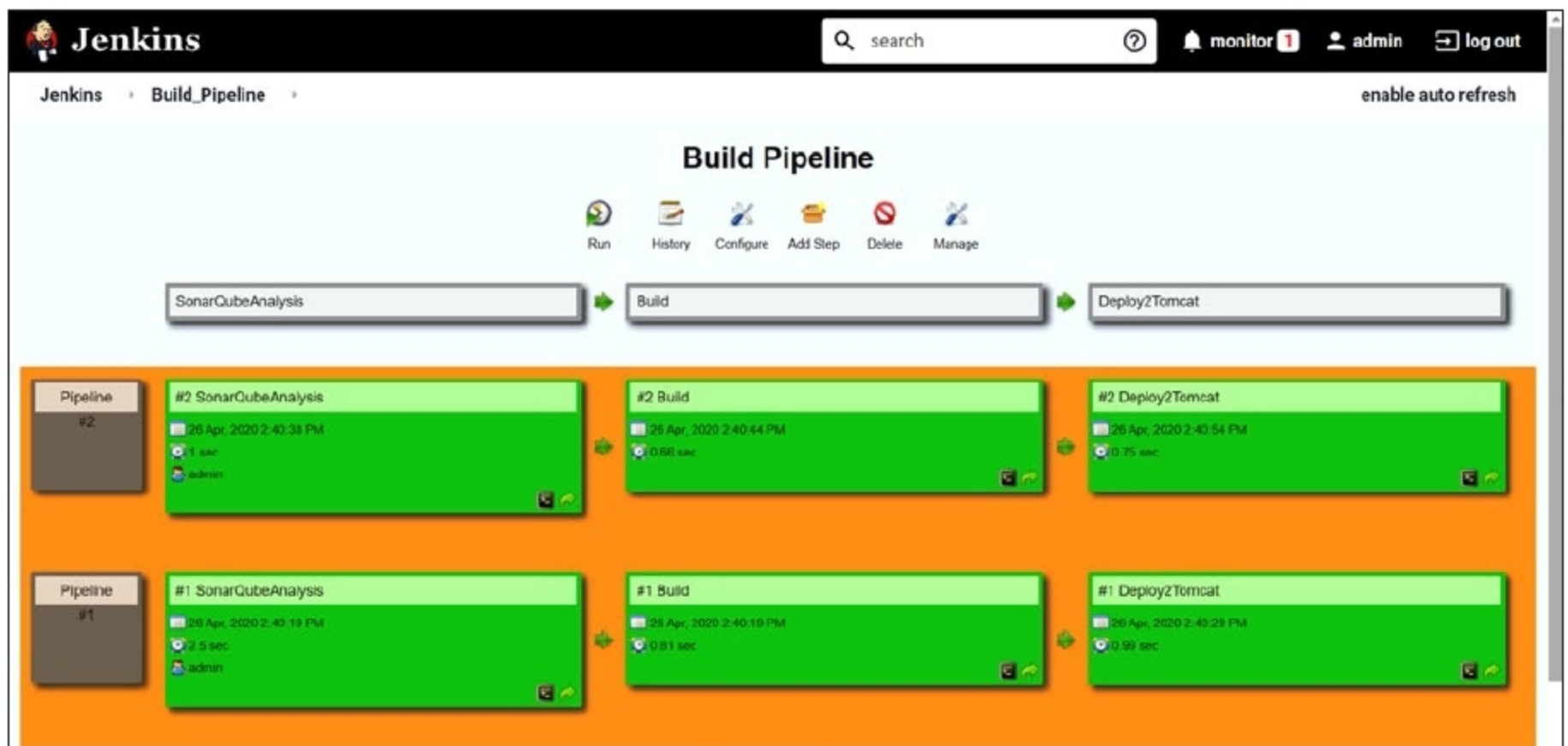
Figure 7: Build Pipeline plugin
