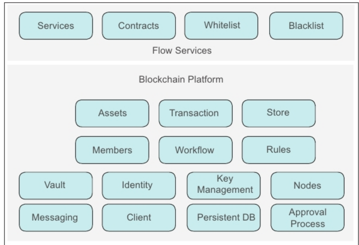
Figure 6: Corda architecture
