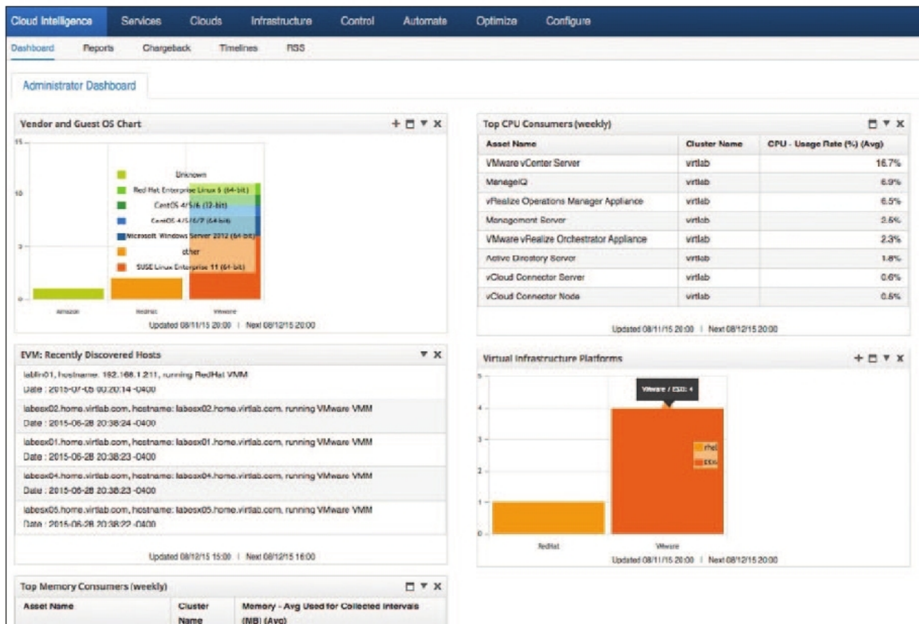
Figure 6: Administrator dashboard
