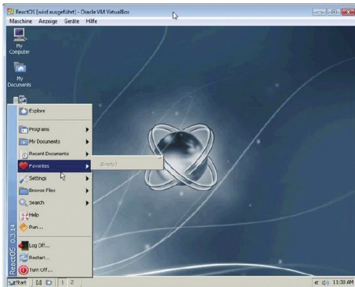
Figure 2: ReactOS
