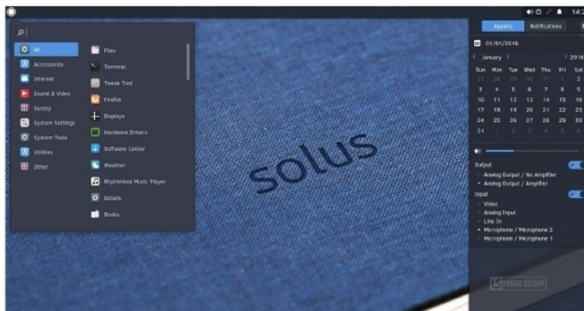
Figure 4: Solus
