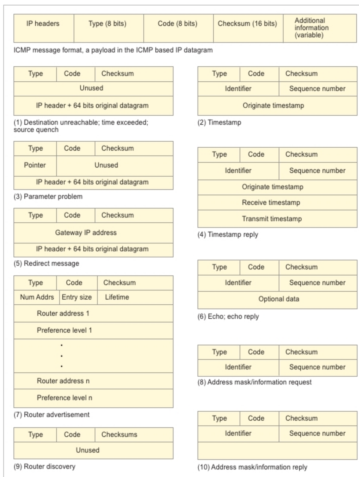
Figure 2: Illustrations of various ICMP message formats
