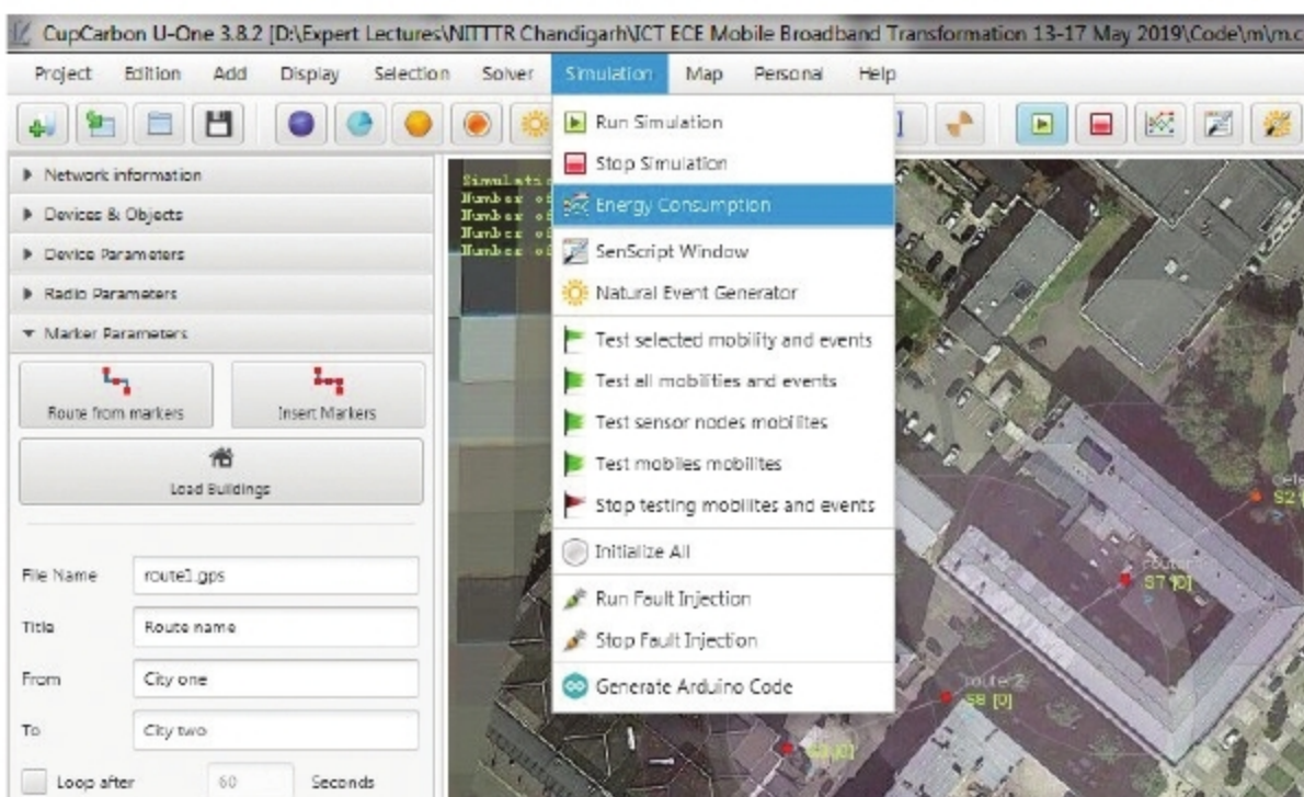
Figure 11: Analysing the energy consumption and research parameters in CupCarbon
