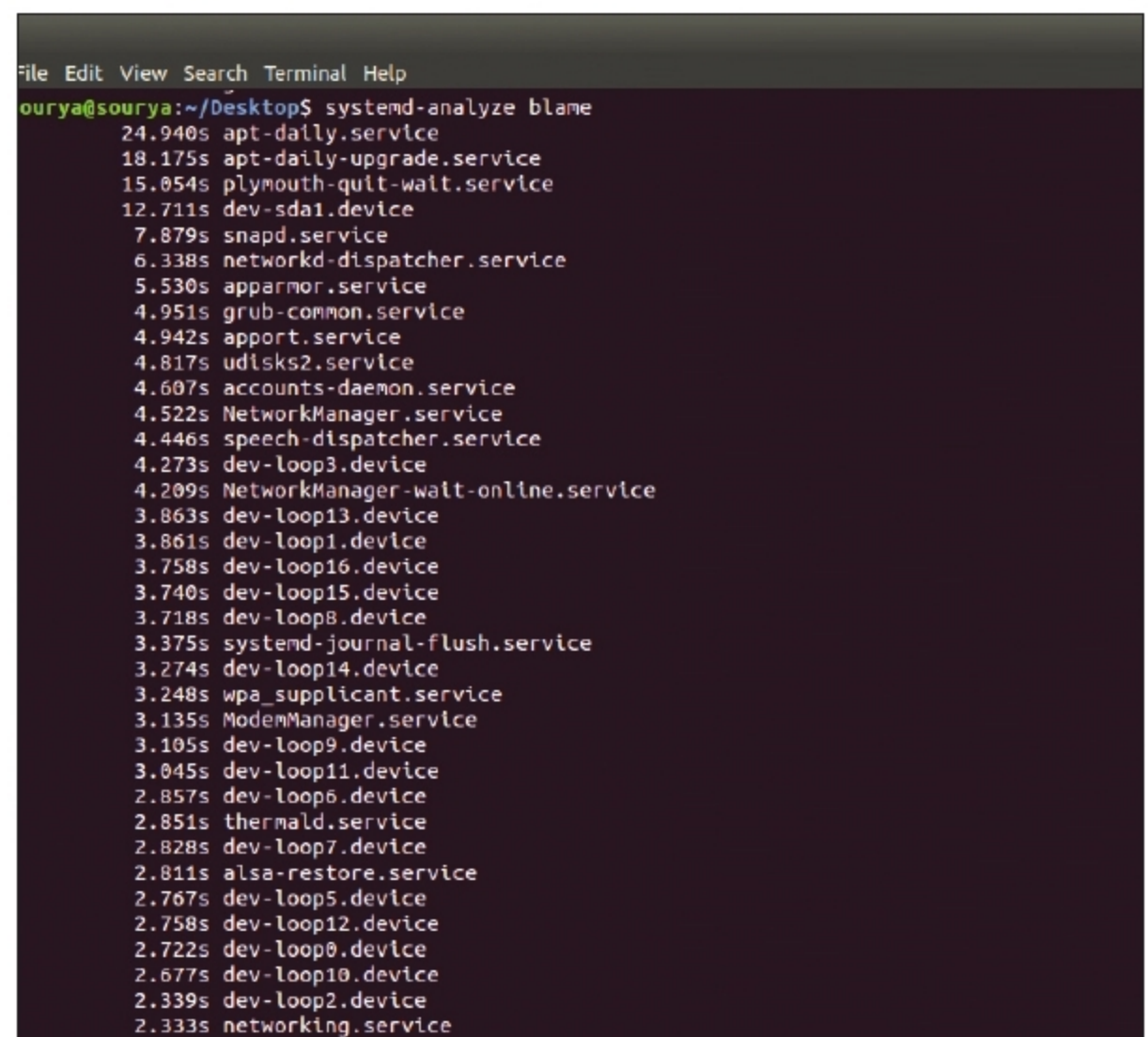
Figure 4: Output of systemd-analyze blame
