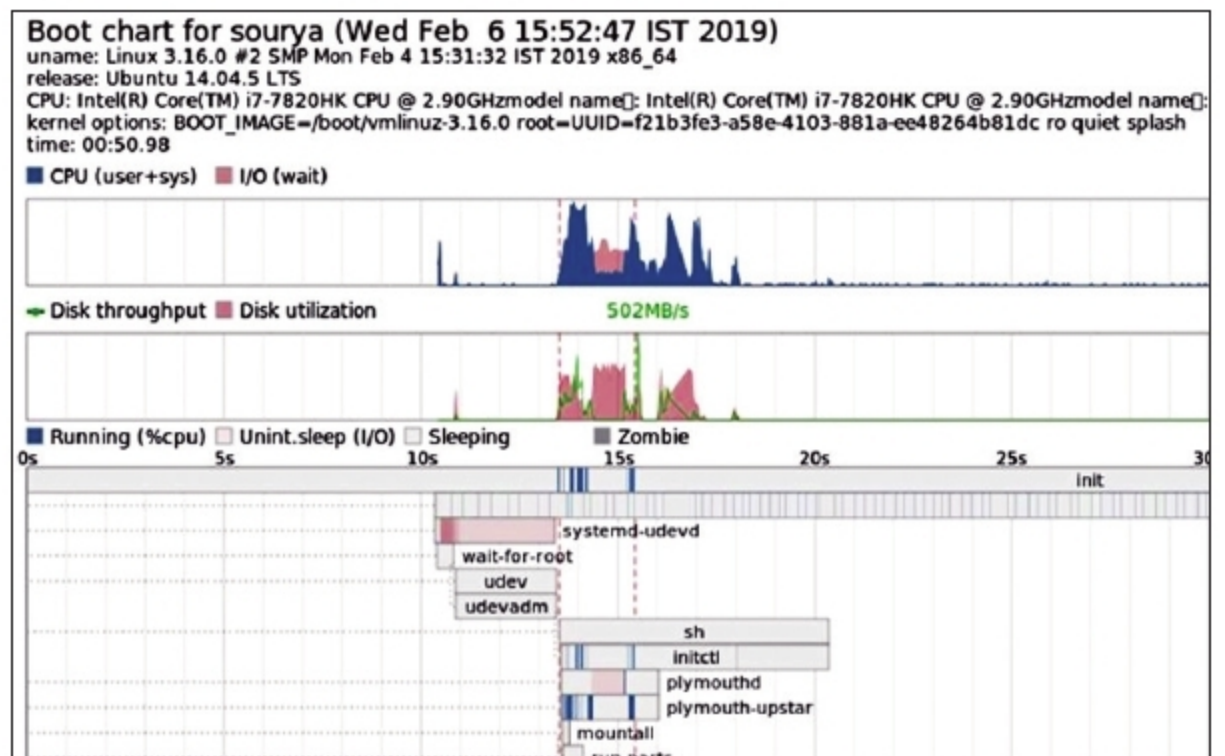
Figure 2: Boot chart
