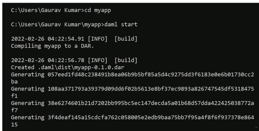
Figure 5: Running DAML
