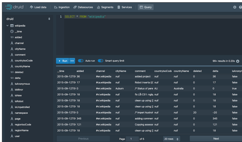
Figure 7: Druid querying
