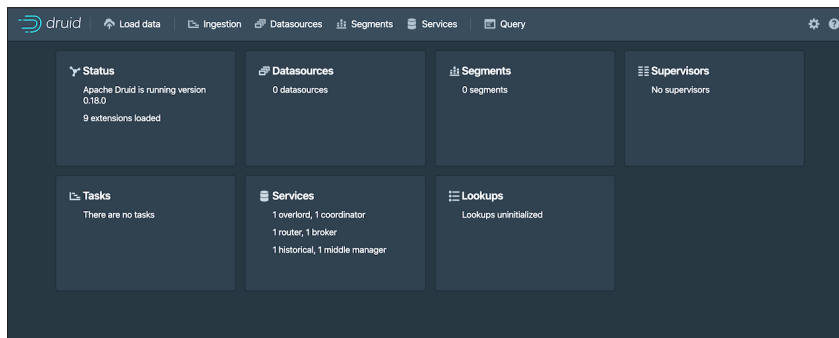
Figure 5: Druid console
