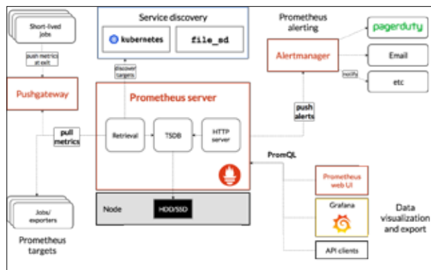
Figure 5: Prometheus architecture
