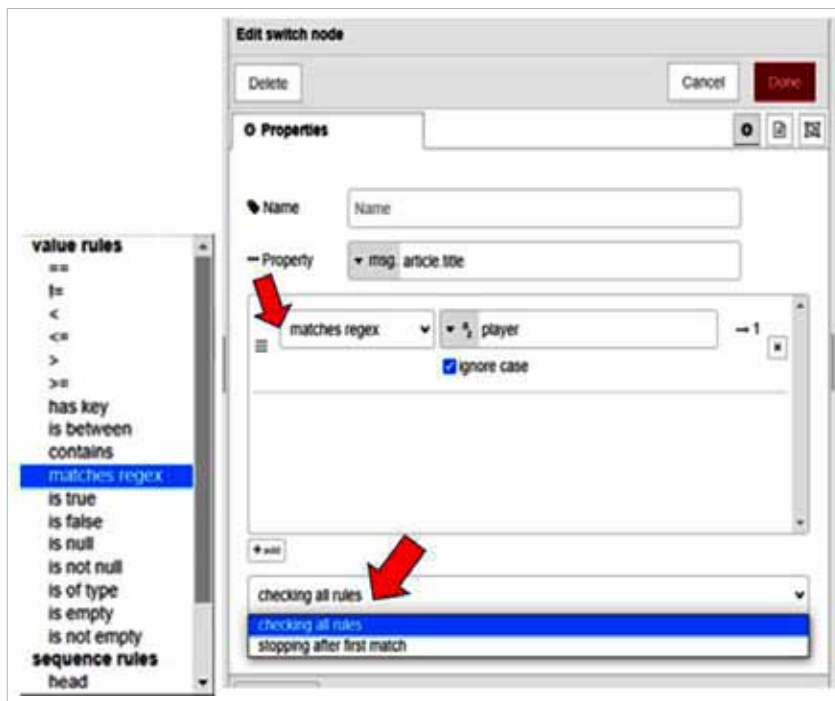
Figure 6: Switch node property configurations
