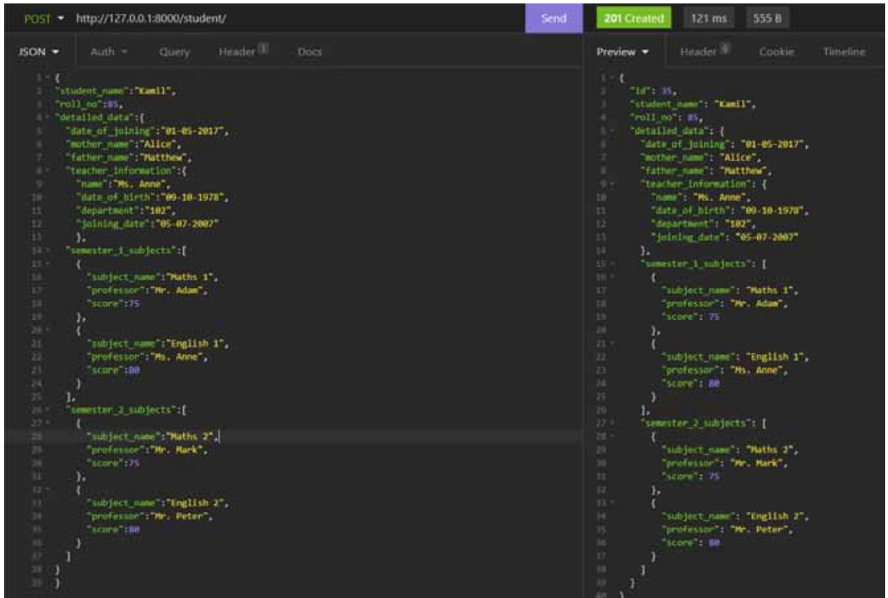
Figure 8: Successful validation of JSONField schema
