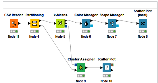
Figure 1: Covid 19 k-means clustering KNIME workflow
