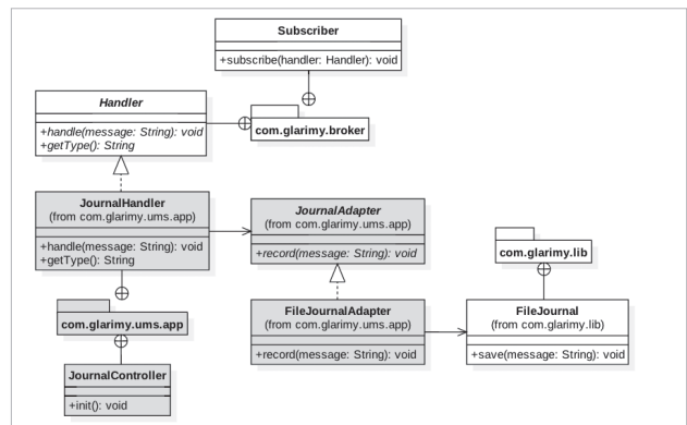
Figure 11: The domain model of JournalService
