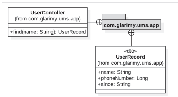
Figure 8: The application layer of FindService
