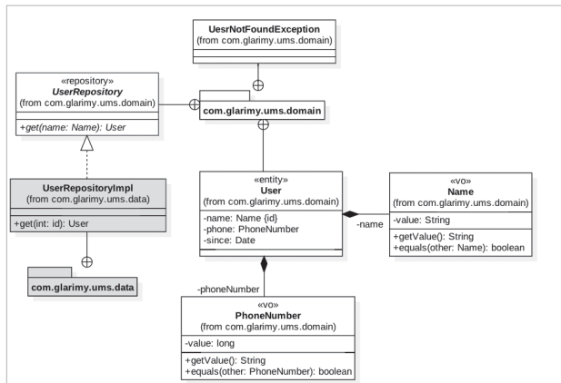
Figure 7: The domain model of FindService
