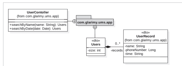
Figure 10: The application layer of SearchService
