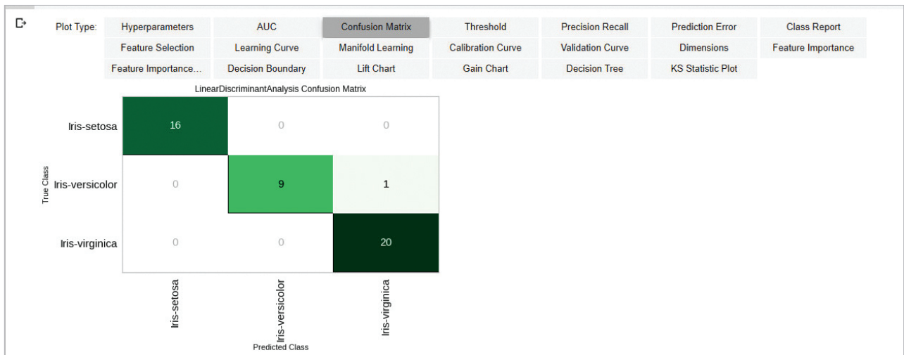
Figure 9: Evaluating and plotting the model performance — confusion matrix
