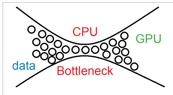
Figure 1: CPU bottleneck
